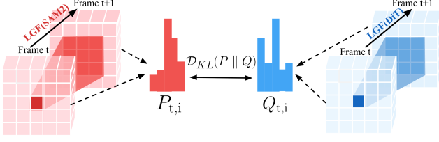
Figure 3. Illustration of the Local Gram Flow (LGF) Loss. The LGF operator captures motion structure by computing similarities between a token at frame t and its 7 \times 7 spatial neighborhood in the subsequent frame t + 1 . Instead of matching absolute values (e.g., \ell_2 ), we convert the resulting similarity vectors ( P_{t,i}, Q_{t,i} ) into probability distributions and align them using the KL Divergence. This forces the model to learn relative motion patterns, not just feature values.
