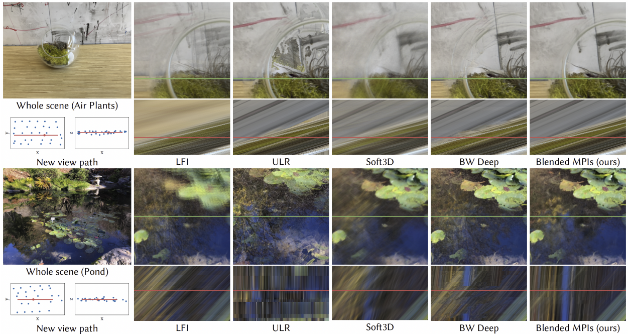
Figure 4: Results on two scenes (from Fig. 9 of the original paper [27]). These datasets were captured by a standard cellphone. We render a sequence of new views and show both a crop from a single rendered output and an epipolar slice of the sequence. We show 2D projections of the input camera poses (blue dots) and new view path (red line) along the z and y axes of the new view camera in the lower left of each row. Comparison is made to prior methods, showcasing the quality of results from local light field fusion.
