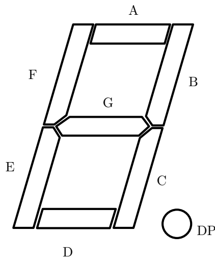
Figure 22.2: 7-Segment Character Segment Mapping
