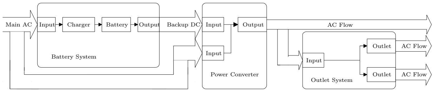
Figure 30.6: A UPS with One Non-Switchable Output and Two Switchable Outlets
