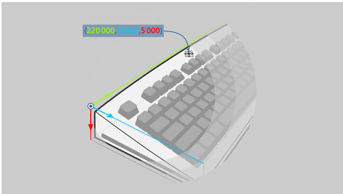
Figure 26.5: Keyboard branding lamp under the logo. Position of lamp relative to the bounding box (described above) labeled in \mu\text{m} .
