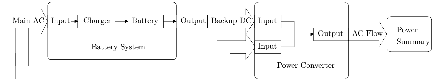
Figure 30.5: A Simple UPS with One Non-Switchable Output
