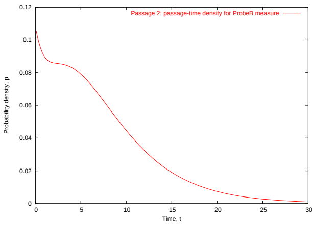
Fig. 2. Average passage-time density for R reads and W writes. ( S = 5 , B = 4 , W = 3 , R = 3 : 69,440 states)
