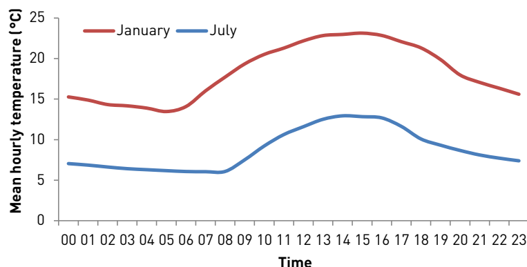
Figure 18. Mean hourly temperatures at Auckland Airport, January and July.
