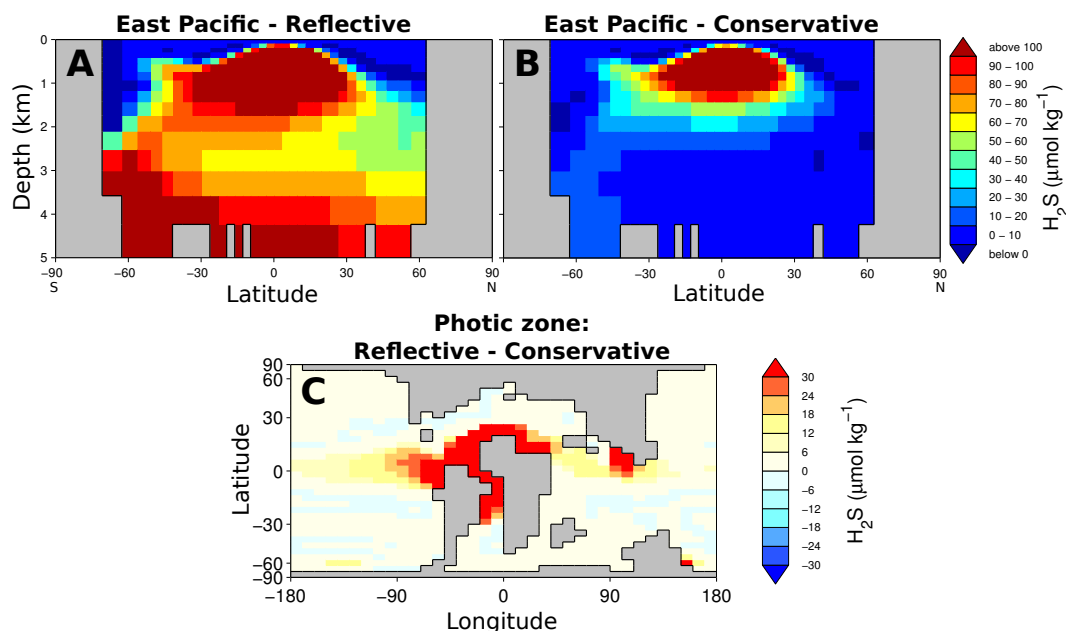
Figure 17: Model comparison of H 2 S concentration during OAE2 with GENIE configurations using the Conservative and Reflective sediment approach. (A+B): Vertical profile of H 2 S in the East Pacific Ocean (−90° longitude). (C): Anomaly plots (Reflective minus Conservative) of photic zone euxina (i.e. H 2 S concentration for 80-200m depth).
