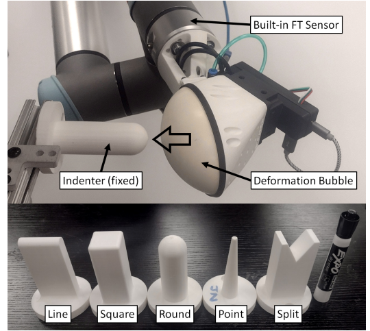
Fig. 4: Photo of the experiment setup. A Punyo sensor is mounted to a UR5 robot, with a built-in force-torque sensor on its end effector. Indenters are mounted to a calibrated, fixed location. The 5 indenters are shown with an EXPO marker for scale. The model was calibrated on 5 trajectories against the Round indenter and one trajectory against the Point indenter, and tested against all five indenters with varying trajectories.
