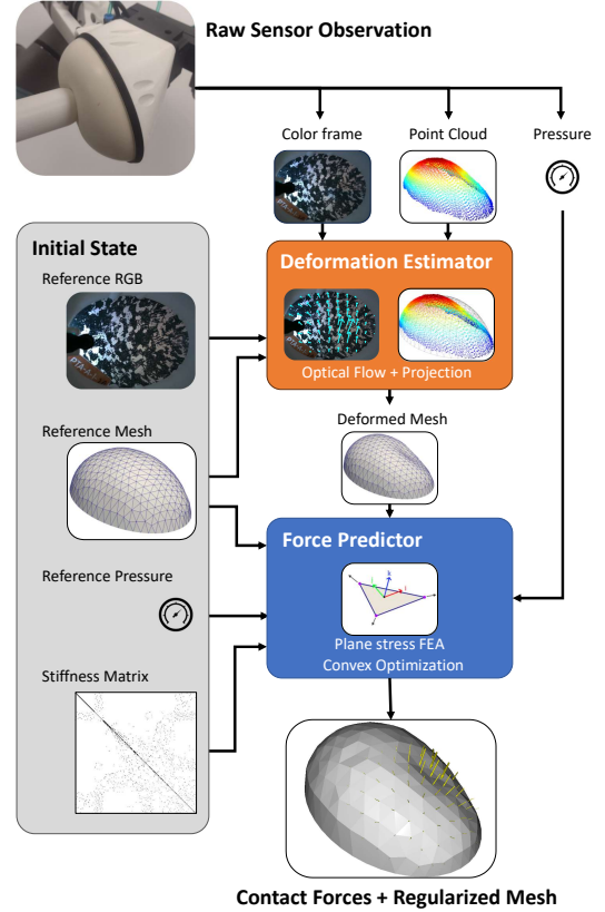
Fig. 1: A summary of the force estimation pipeline. An RGB image and point cloud from the bubble sensor are used to estimate the 3D mesh deformation relative to a reference configuration. We construct a finite element model of the bubble to predict forces from observed deformations and pressure changes. A convex optimization problem combines the physics model and camera observations, giving contact force estimates and regularizing the raw observations.
