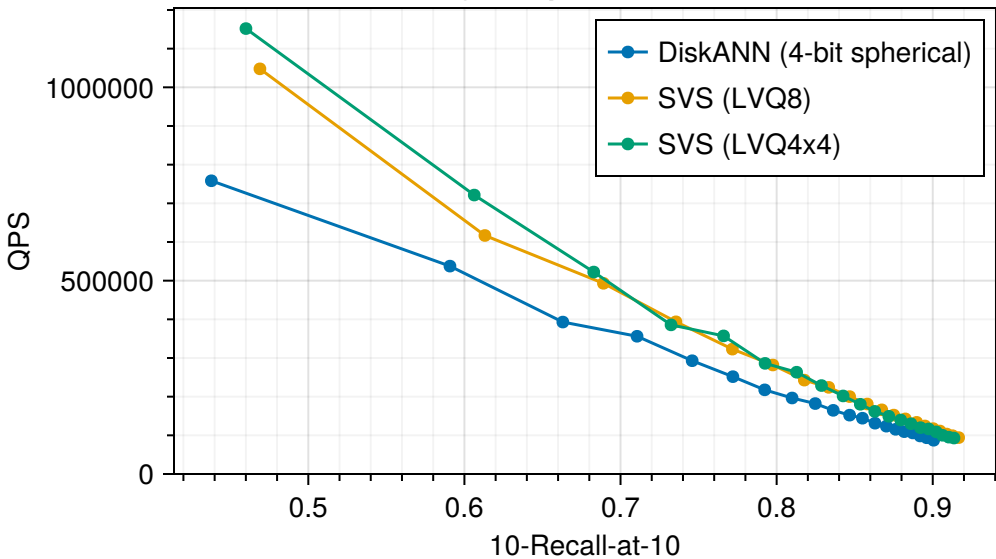
MSTuring-1M, quantized, 32 threads
