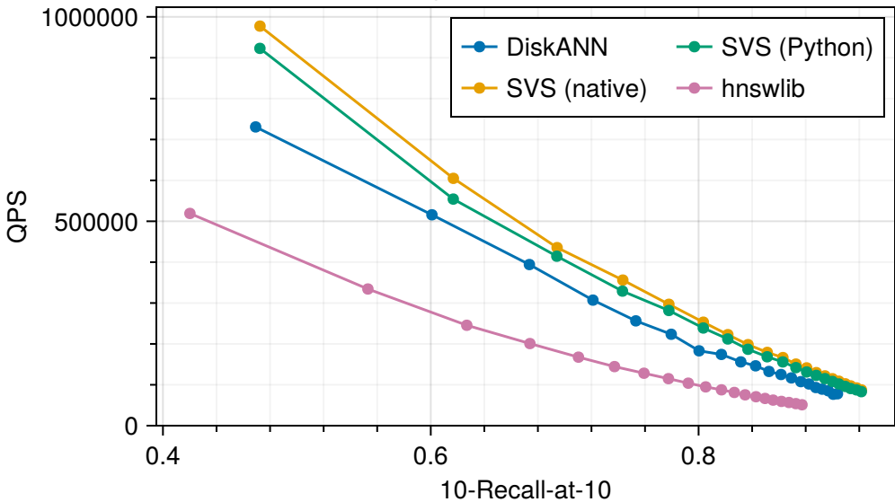
MSTuring-1M, float32, 32 threads
