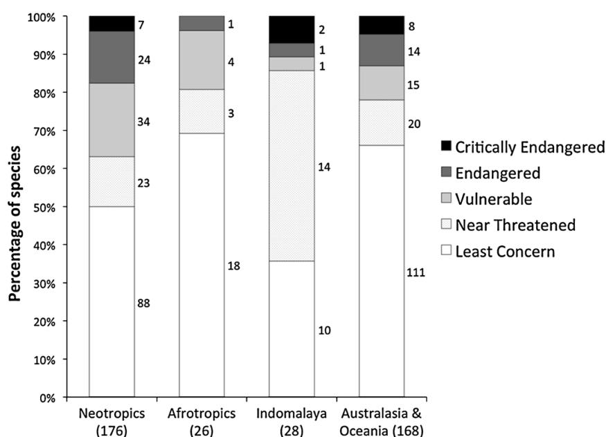
Fig. 2 Proportion of parrot species in each IUCN Red List category for each region (following Croxall et al. 2012). Number of species in each category is shown
