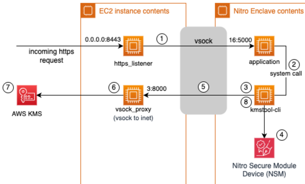
Figure 2: Decrypt with AWS KMS and cryptographic attestation
