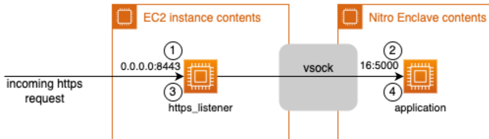
Figure 1: vsock language binding
