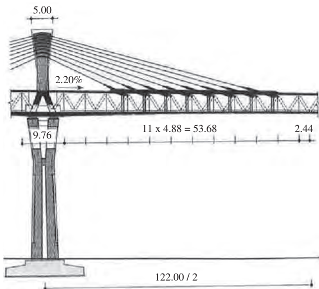
Figure 2.16: Povazska Bridge 37
