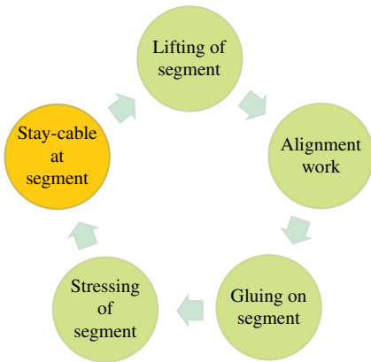
Figure 6.35: Erection work flow
