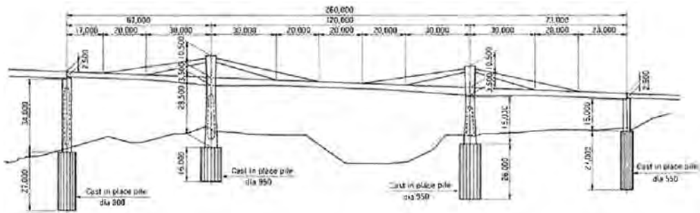
Figure 2.25: Okuyama bridge 44
