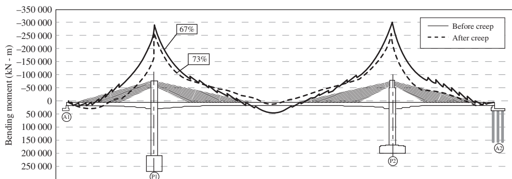
Figure 3.5: Bending moment under dead load (Tsukuhara Bridge)
