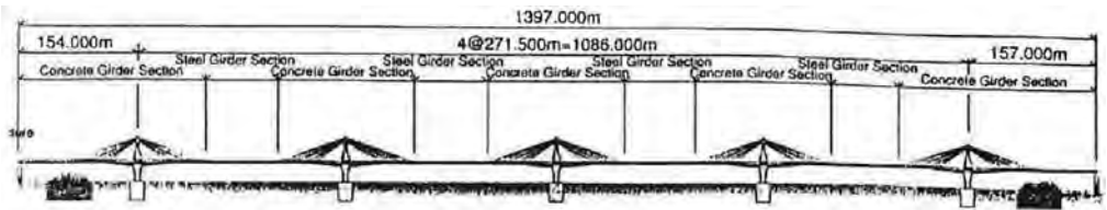
Figure 2.13: Ibigawa Bridge 35
