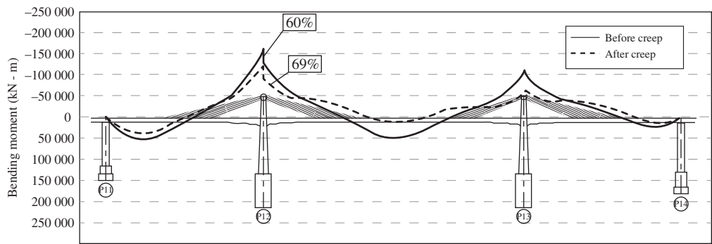
Figure 3.4: Bending moment under dead load (Odawara Blueway Bridge)
