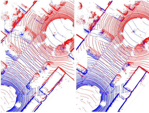
Fig. 3. Successful registration of two lidar spins, taken from the KITTI odometry dataset [34]. On the left, the initial registration from the RTK GPS poses. On the right, the registration refined by HMRF ICP. No information about the data topology was used.
