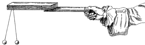
Figure 6.38: Canton's electroscope.
