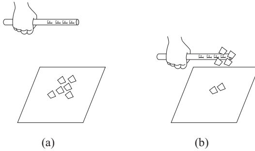
Figure 2.3: (a) A rubbed straw far away from small pieces of paper. (b) The rubbed straw attracts the pieces of paper when brought close to them.
