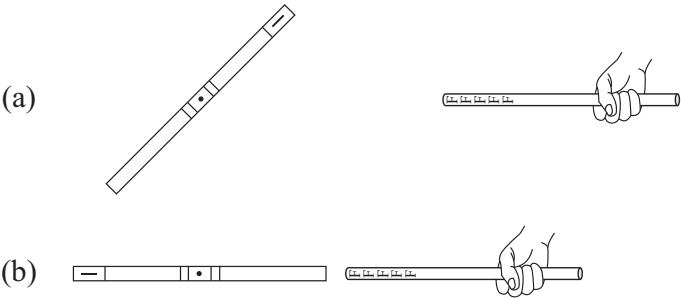
Figure 5.23: Negatively charged aluminum foil of a Du Fay versorium being repelled by an electrified body approaching it.
