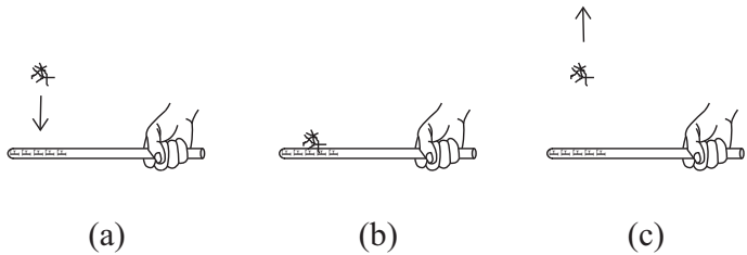
Figure 4.4: (a) A piece of cotton is initially attracted by a rubbed plastic straw. (b) The cotton touches the rubbed portion of the straw. (c) After contact, the cotton is repelled by the straw. It can then be kept floating above the straw despite the gravitational attraction of the Earth!
