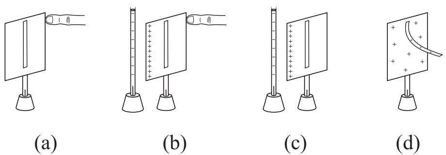
Figure 7.22: Distribution of charges of Figure 7.21.
