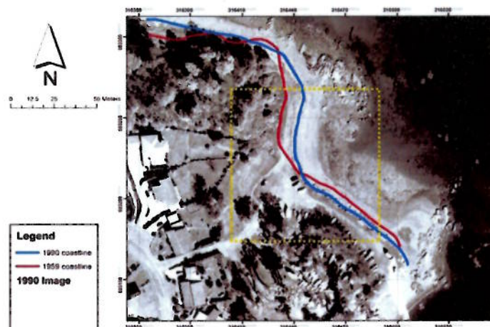
c. Coastline changes in the Boatyard and "Mud" bay area, 1955 to 1990
