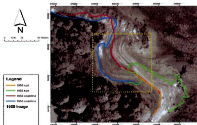
b. Coastline changes in the Boatyard and "Mud" bay area, 1955 to 1959
