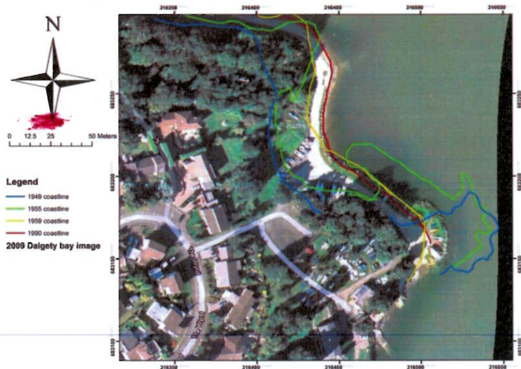
Figure 2.4 Shoreline contours for the east of the study area, the Boatyard and 'Mud' Bay area.
