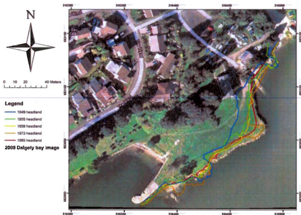
Figure 2.3 Shoreline contours for the west of the study area, the 'headland' area.
