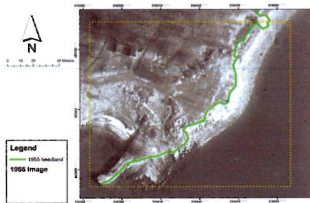
b. The coastline of the Headland area in 1955
