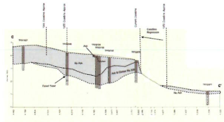
b. Cross section through the coastline and beach along line CC' in Figure 7.1
