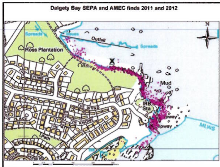
Figure 4.1 Map of the Dalgety Bay site showing the distribution of radioactive items found by MoD and SEPA surveys in 2011 and 2012 (SEPA, 2013).
