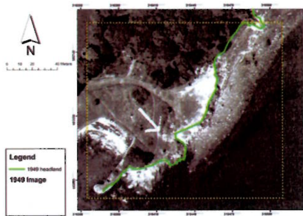
a. The coastline of the Headland area in 1949
