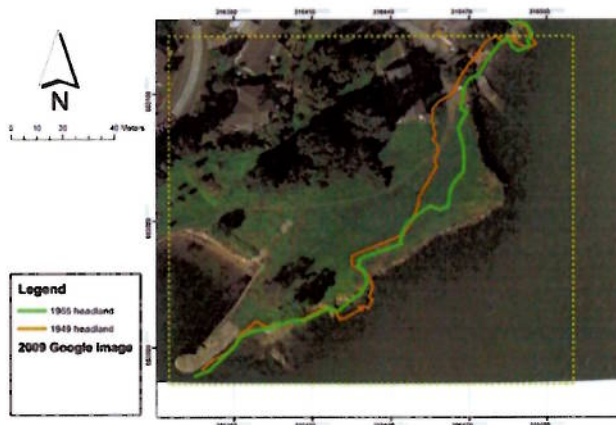
c. A comparison of the 1949 and 1955 coastlines with the Headland in 2009
