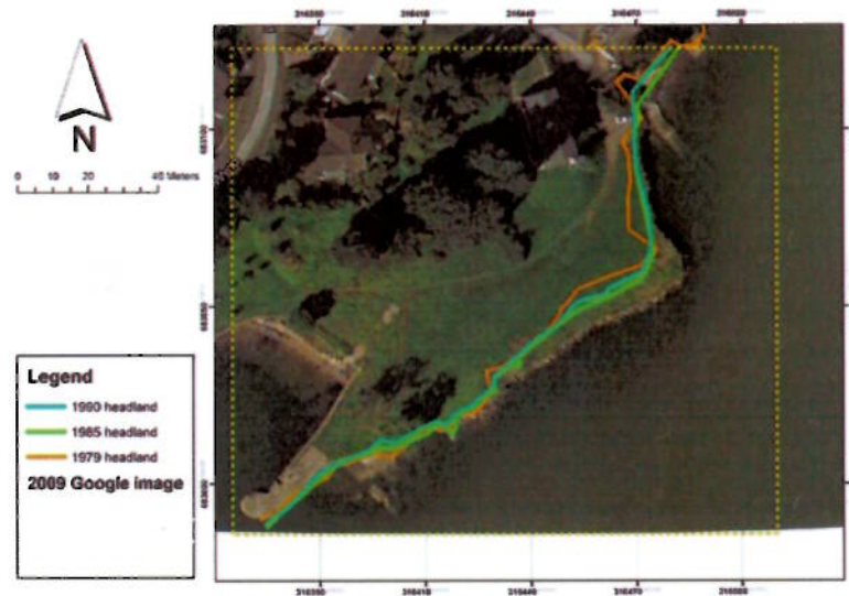
a. Coastline changes in the Headland area since 1979
