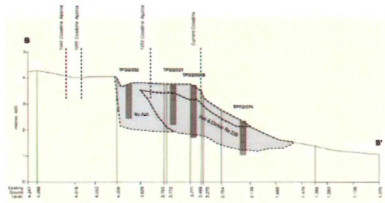
a. Cross section through the coastline and beach along line BB' in Figure 7.1
