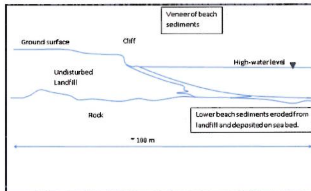
Figure 7.2 : Conceptual cross-section of part of the landfill and adjacent beach (not to scale).
