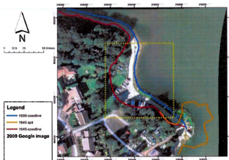
b. Coastline changes in the Boatyard and "Mud" bay area since 1945
