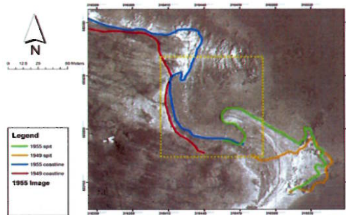
a. Coastline changes in the Boatyard and "Mud" bay area, 1949 to 1955
