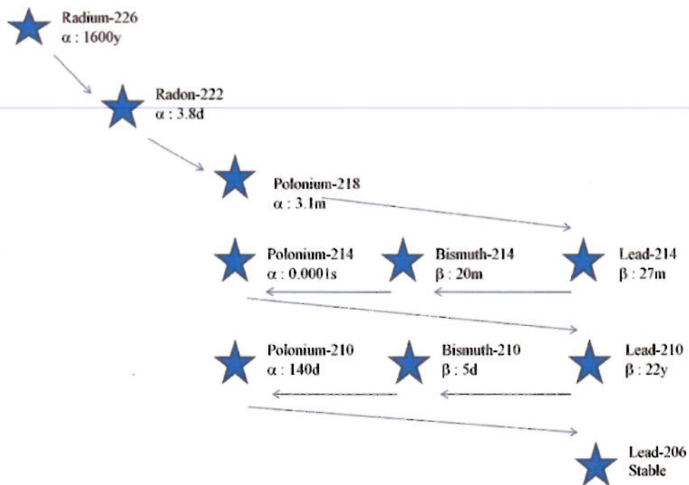
Figure 3.1 Decay chain of radium-226, showing radionuclide, type of radioactive decay and physical half-life
